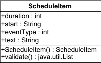
Figure 12.2 UML notation for a class shows the name at the top, the attributes (properties) in the middle, and the operations (methods) at the bottom.
