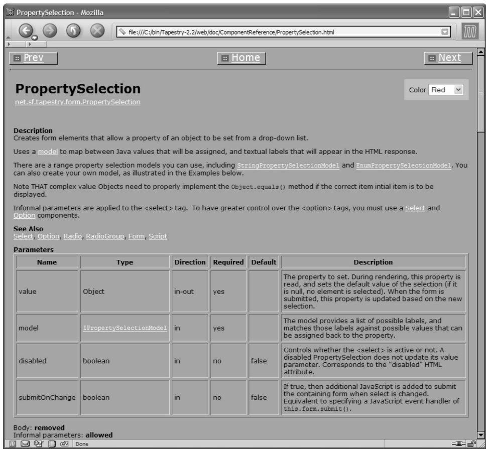
Figure 6.10 The additional Component Reference pages are critical for the page specifications and for using the full features of the components.
