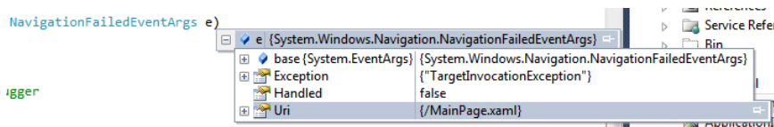
Figure 4–5. NavigationFailedEventArgs.Uri
