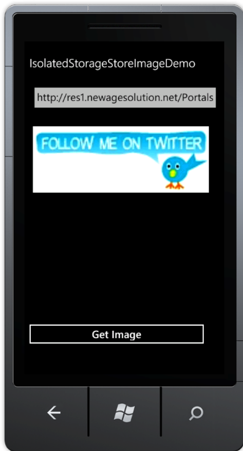
Figure 13–2. IsolatedStorageStoreImageDemo
