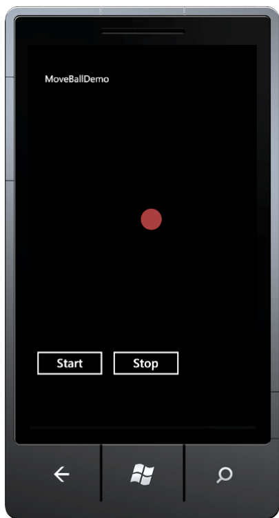
Figure 6–15. MoveBallDemo UI
