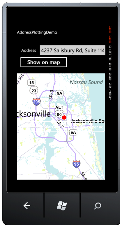
Figure 14–9. AddressPlottingDemo application
