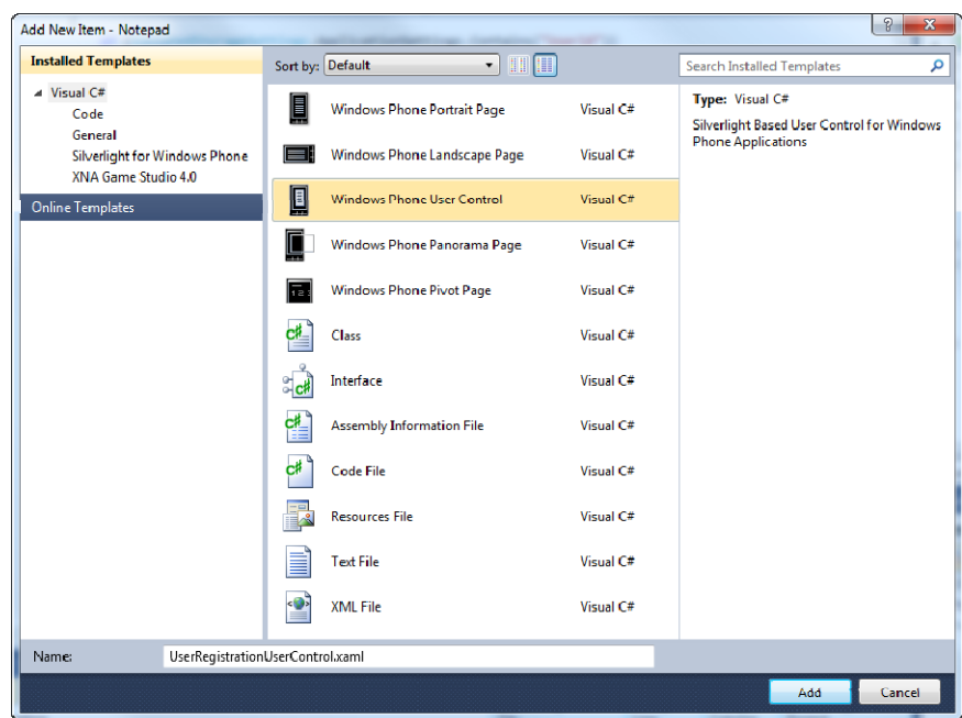
Figure 3–29. Creating UserRegistrationUserControl
