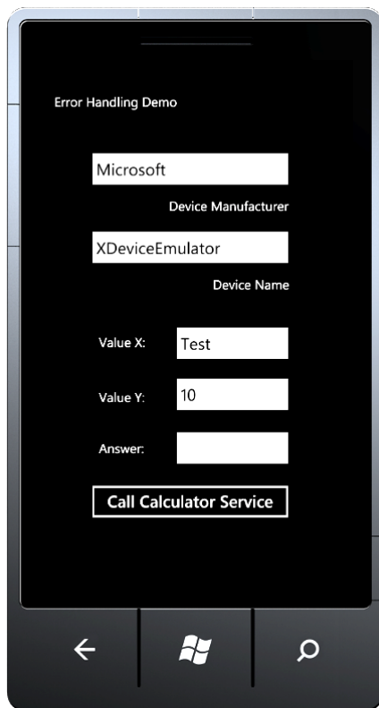
Figure 4–1. ErrorHandlingDemo application
