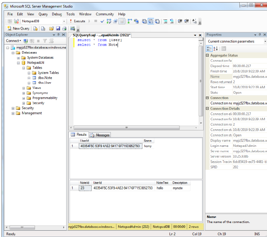
Figure 3–35. Querying NotepadDB
