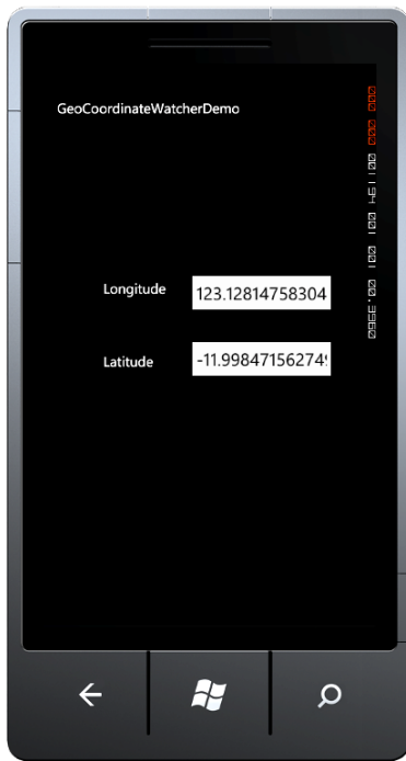
Figure 14–3. GeoCoordinateWatcherDemo
