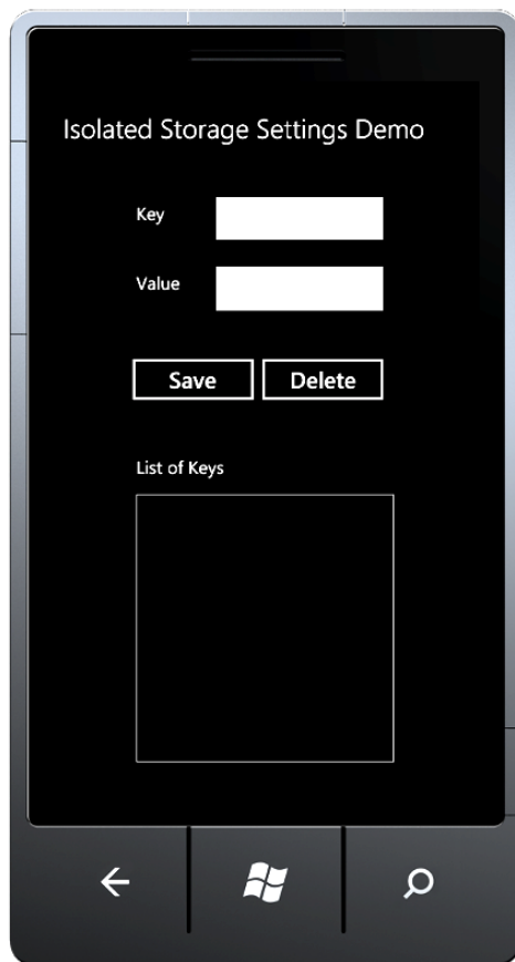
Figure 13–5. IsolatedStorageSettingsDemo
