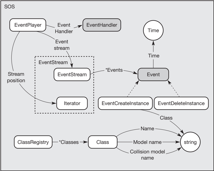
Figure 11.5 The scenery object streaming (SOS) component.
