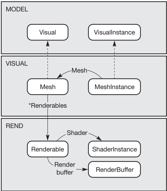
The VISUAL component is shown in Figure 5.23.
