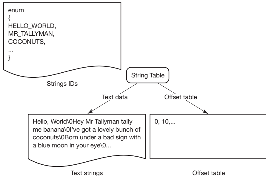
Figure 5.16 The constituents of a string table.
