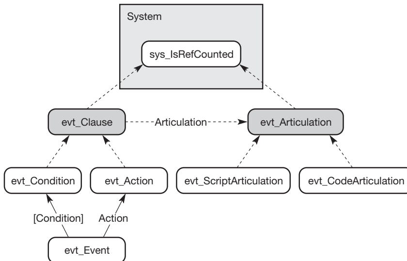
Figure 8.4 Event system part 1.
