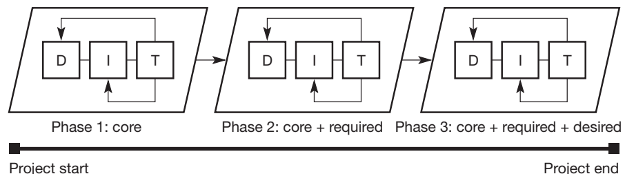
Figure 10.5 Iteration over the three development phases.
