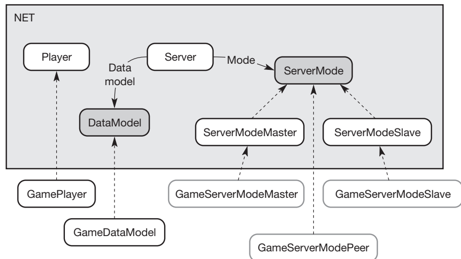
Figure 5.50 Game implementations of abstract or overridable behaviours in the NET component.
