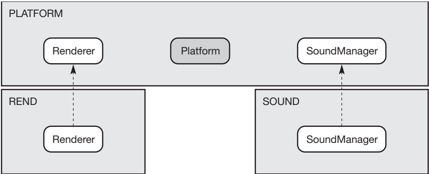
Figure 6.7 Object diagram for platform-independent renderer and sound manager.
