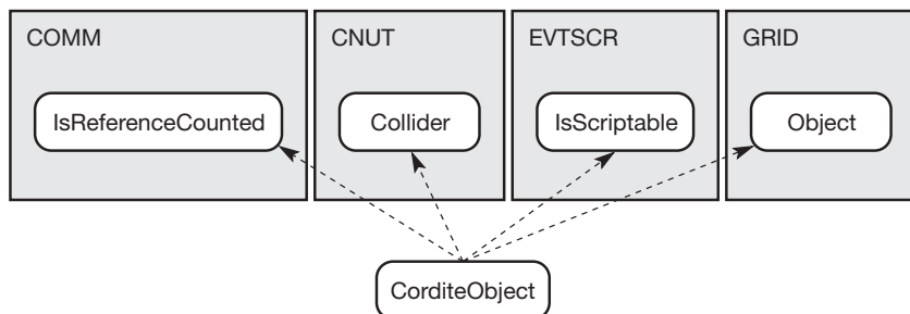
Figure 11.10 Cordite objects are created with the multiple inheritance mix-in method.
