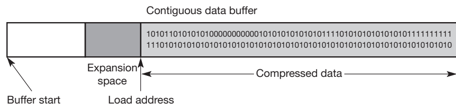
Figure 5.36 Decompressing data on top of themselves.
