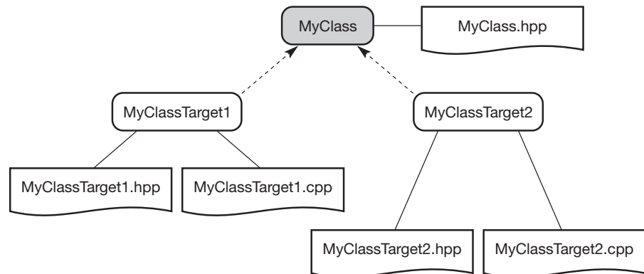
Figure 6.2 Cross-platform class hierarchy.
