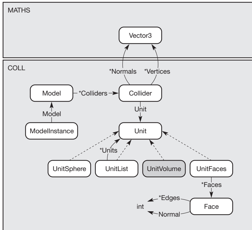
Figure 5.26 The COLL component.
