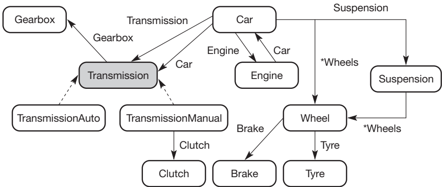
Figure 4.1 Class diagram for a basic car.
