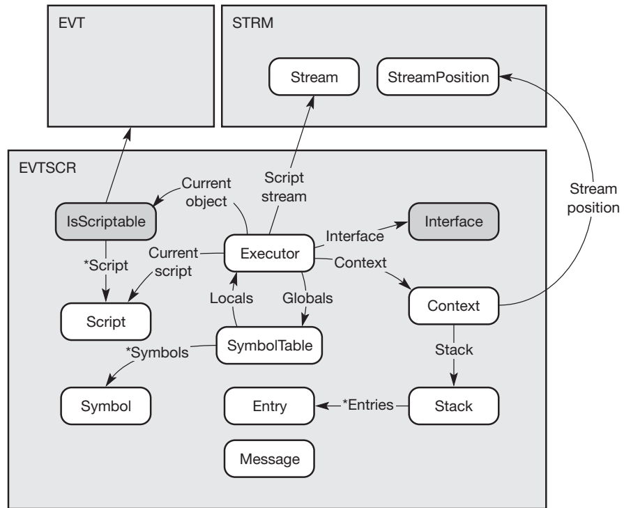
Figure 11.9 The scripted event (EVTSCR) component.
