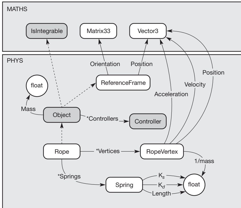
Figure 5.46 Adding ropes to the physics component.
