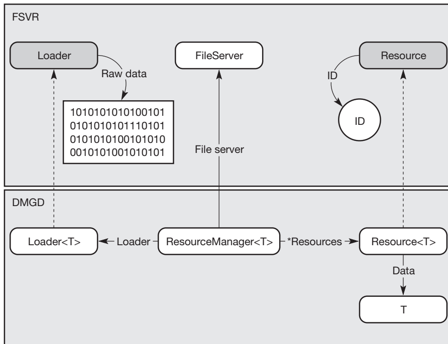
Figure 5.32 DEMIGOD and the file server component diagrams.
