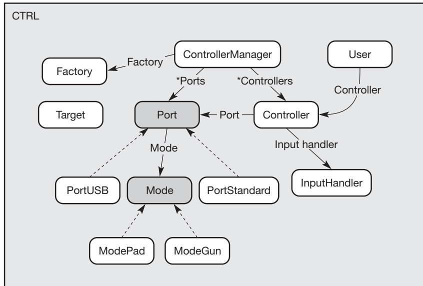
Figure 11.14 The CTRL controller component.
