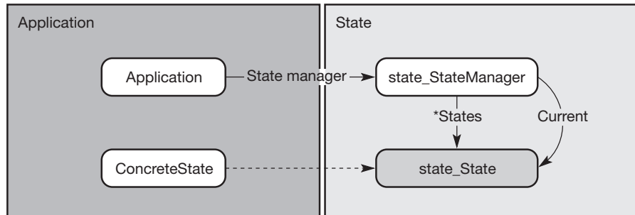
Figure 4.10 The application implements concrete versions of the abstract state class.
