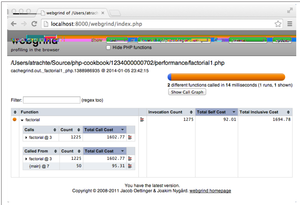
Figure 22-3. Inspecting profiling results in Webgrind
