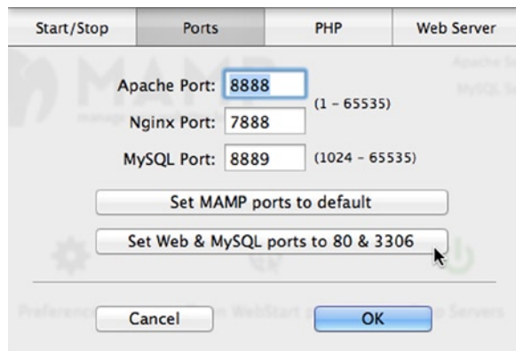
Figure 2-2. Changing the Apache and MySQL ports
