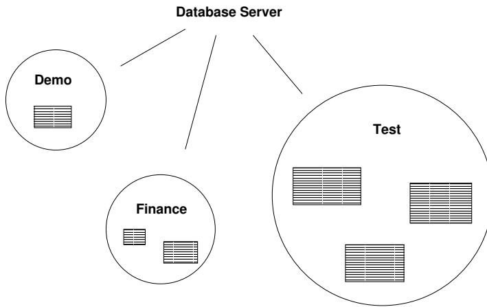
Figure 3.1: Databases
