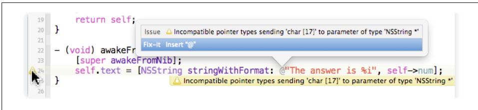
Figure 9-3. A warning with a Fix-it suggestion
