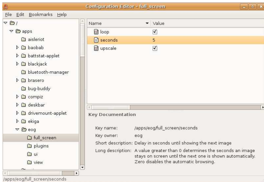
Figure 2.12: gconf-editor
